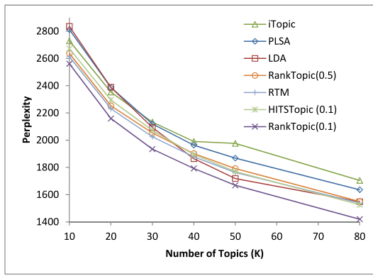
(a) Perplexity Comparison on ArnetMiner
