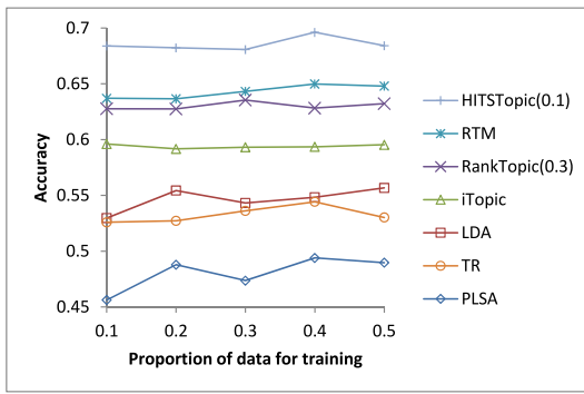
(a) Classification on Citeseer
