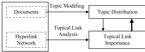
Fig. 3. Mutual enhancement framework between topic distribution and link based importance.
