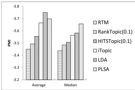
Fig. 14. The average and median PMI values of topics detected by different topic models. The lower the bar, the better topic interpretability. For RankTopic and HITSTopic, PMI for \xi = 0.1 is only shown.
