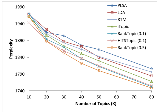
(b) Perplexity Comparison on Twitter
