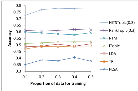
(b) Classification on Cora
