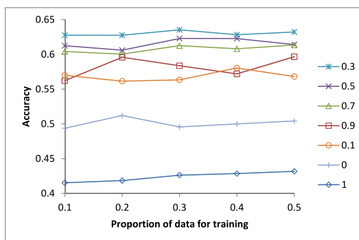
Fig. 11. Classification accuracy of RankTopic with some typical values of \xi on Citeseer data set for different proportions of training data. Accuracy is defined as the fraction of the correctly classified documents to the total number of documents. The higher the accuracy, the better the classification quality.
