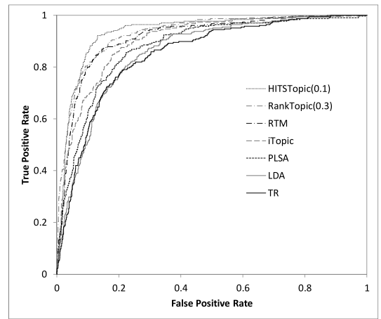
Fig. 13. ROC of different topic models for the first class of Citeseer data.
