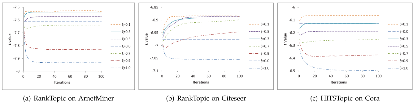
Fig. 5. L curves of LIMTopic with the iterations.
